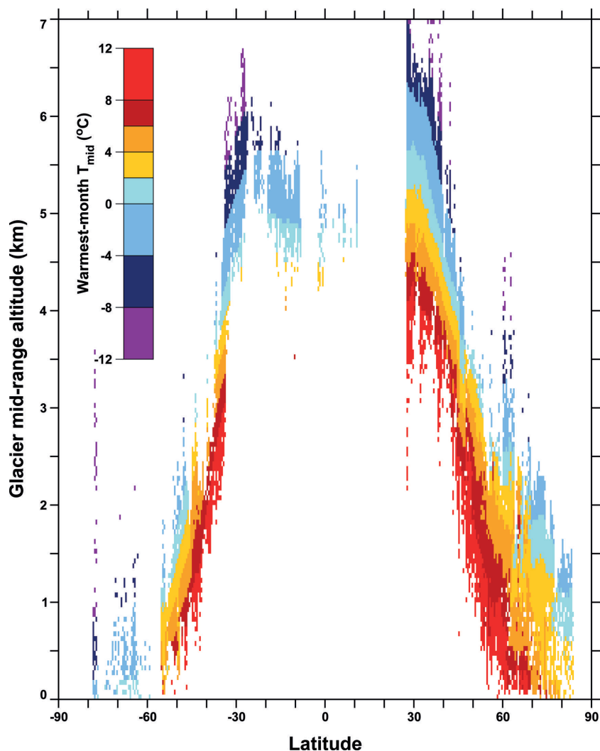
Fig. 10. Zonal averages of the mean temperature of the warmest month at the glacier mid-range altitude (the average of the minimum and maximum glacier altitude). RGI glaciers with minimum altitudes of zero, assumed to be tidewater glaciers, were discarded. The mid-range altitude of each remaining glacier was estimated by overlaying its outline on a suitable DEM (see Radić and others, 2014, for details). The altitudes were averaged firstly into cells of size 50\text{m} \times 0.5^\circ \times 0.5^\circ and then over longitude. Temperatures are warmest-month free-air temperatures interpolated from the US National Centers for Environmental Prediction (NCEP)/National Center for Atmospheric Research (NCAR) Reanalysis (Kalnay and others, 1996).
